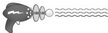
Incoherent Waves
